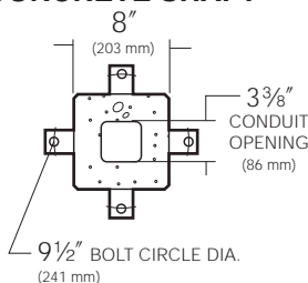
BASE PLAN VSB CONCRETE SHAFT
