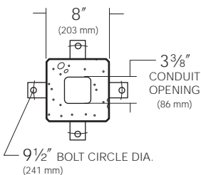
BASE PLAN VSB CONCRETE SHAFT
