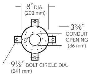
BASE PLAN VRB CONCRETE SHAFT
