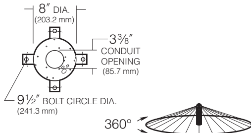
BASE PLAN VRB CONCRETE SHAFT
